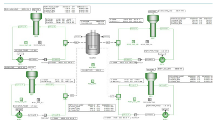
Figure 1: Reactor Process Flow Diagram (from DVR model)
